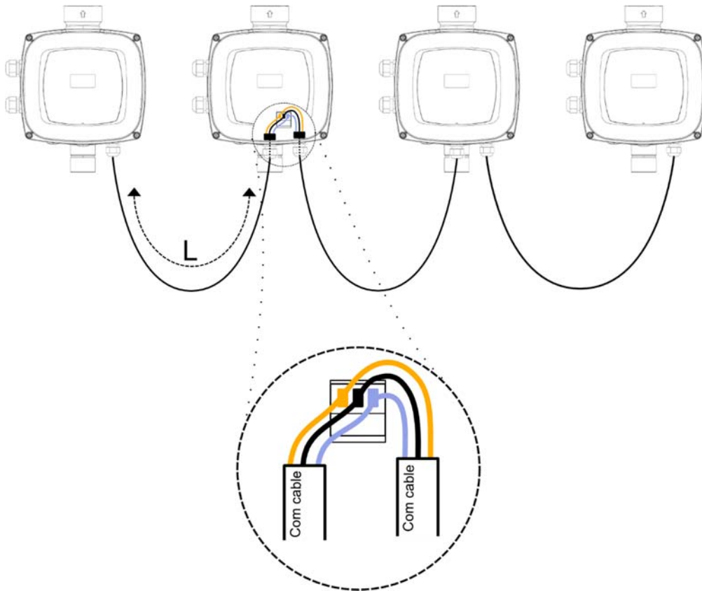
Figure 4: Example of connection of the multi-inverter communication with 4 devices
