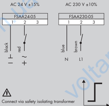
Wiring diagram FSAA24/230-05
