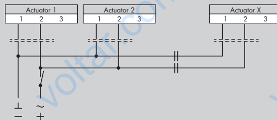
Wiring diagram for parallel operation FSAA24/230-05
