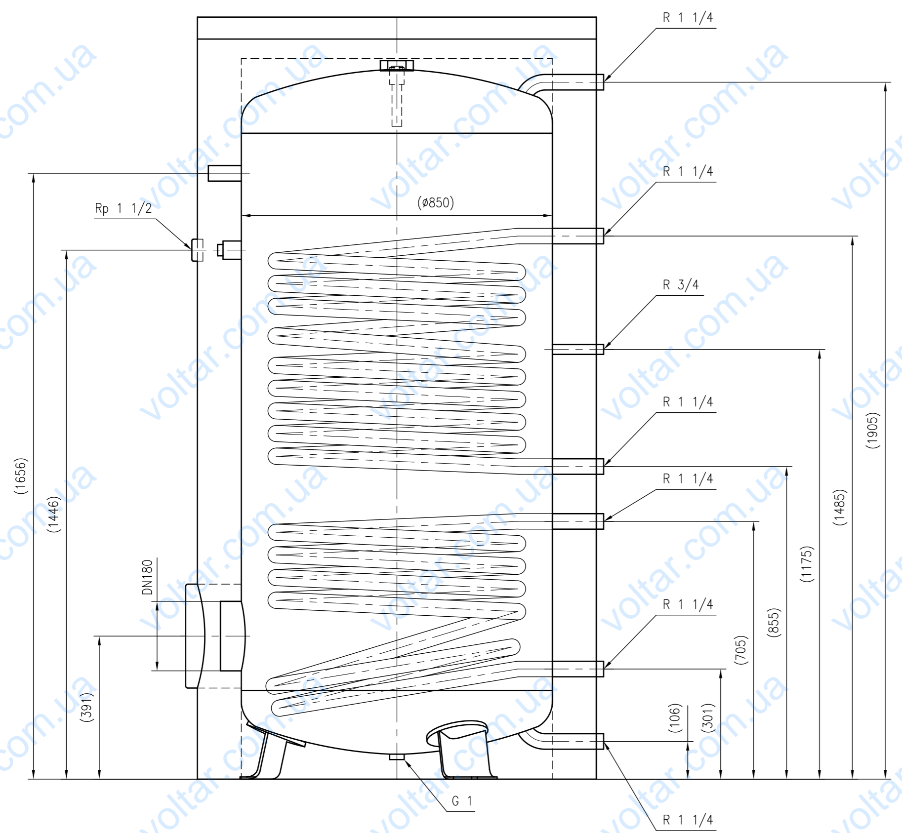
Side view
