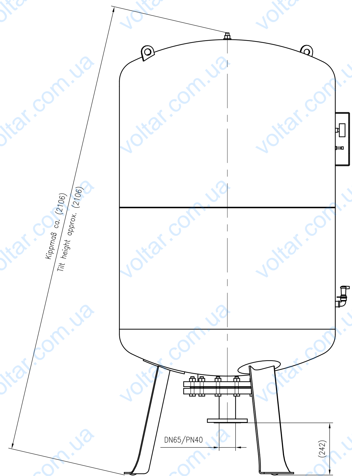
Side view
