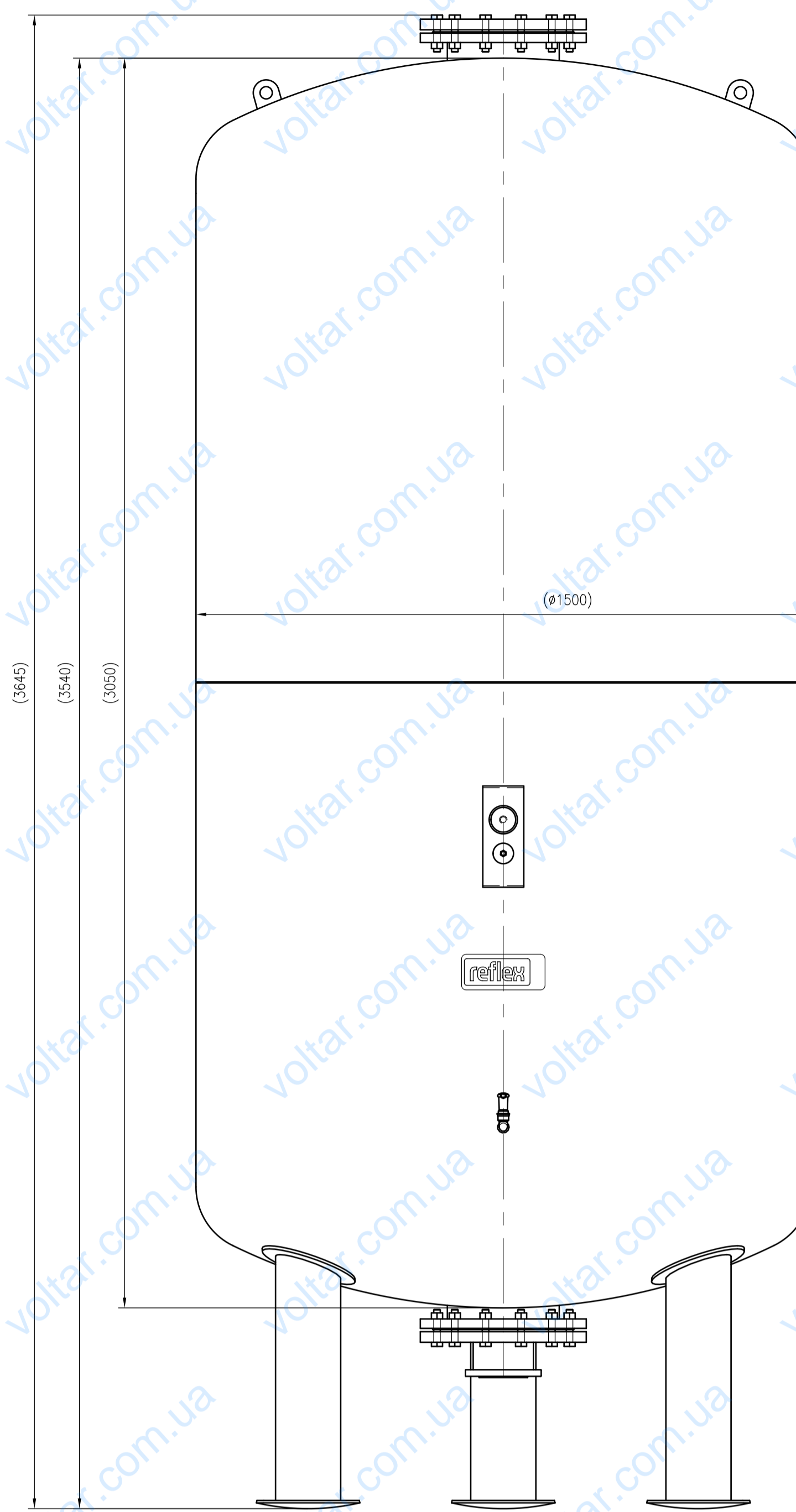
Front view
