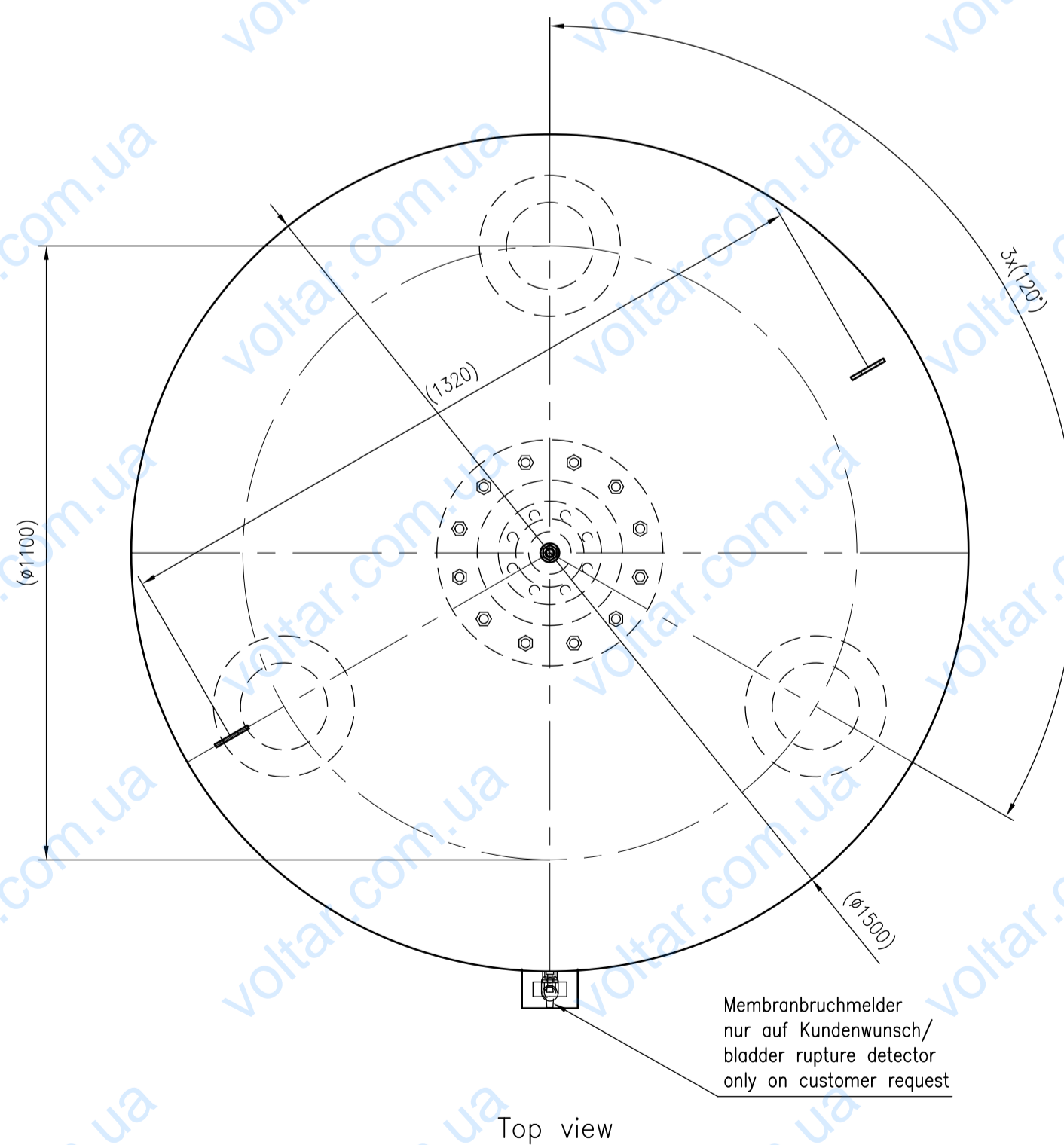
Top view
