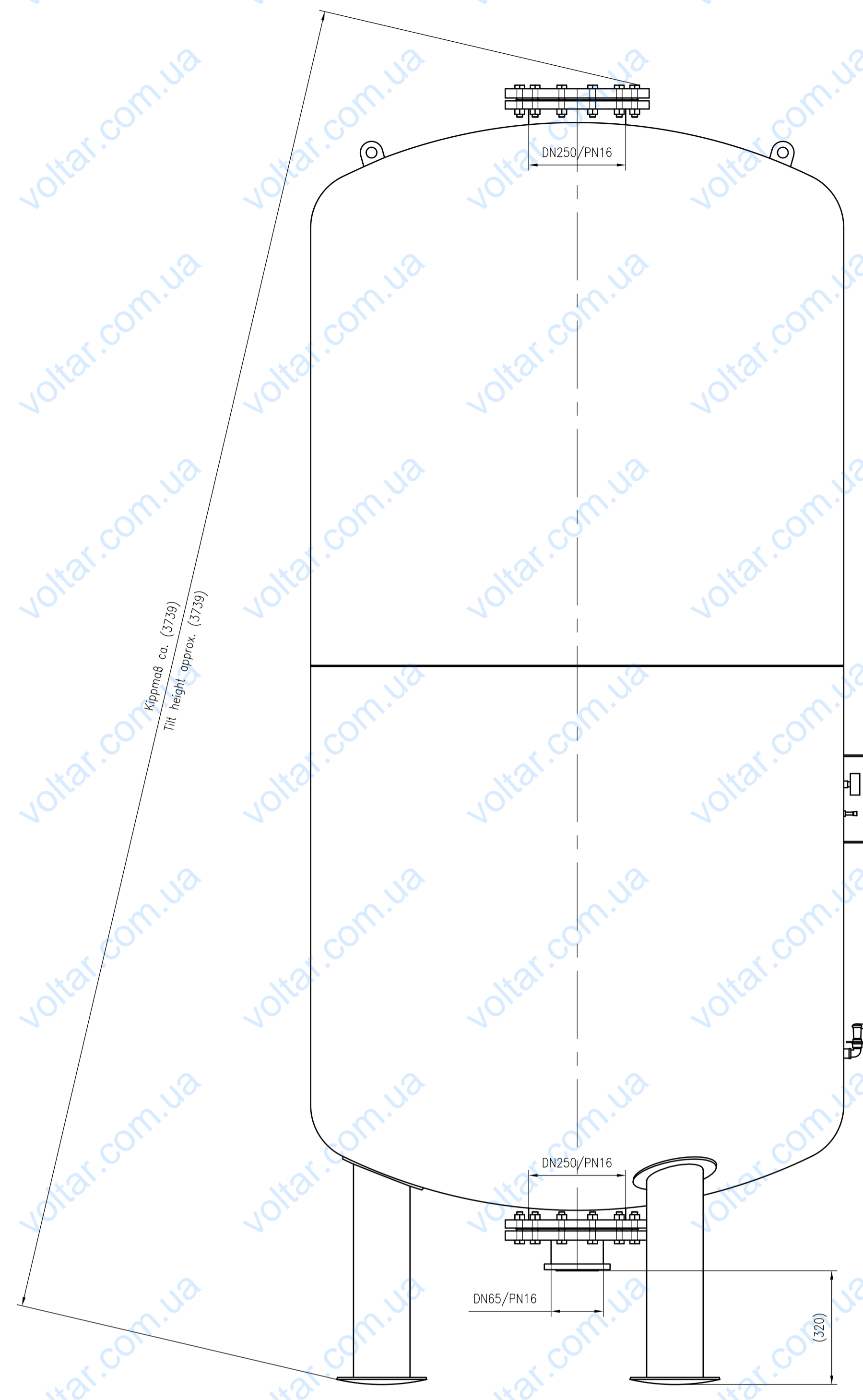
Side view
