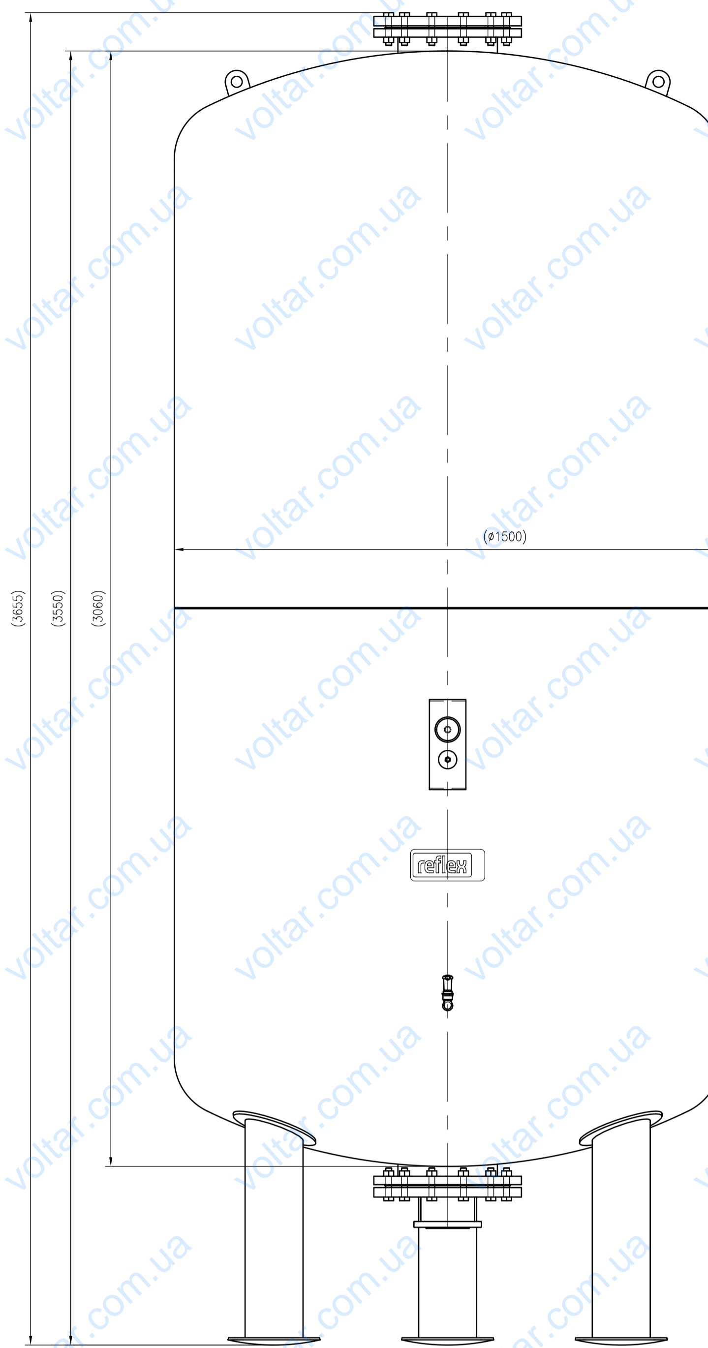
Front view
