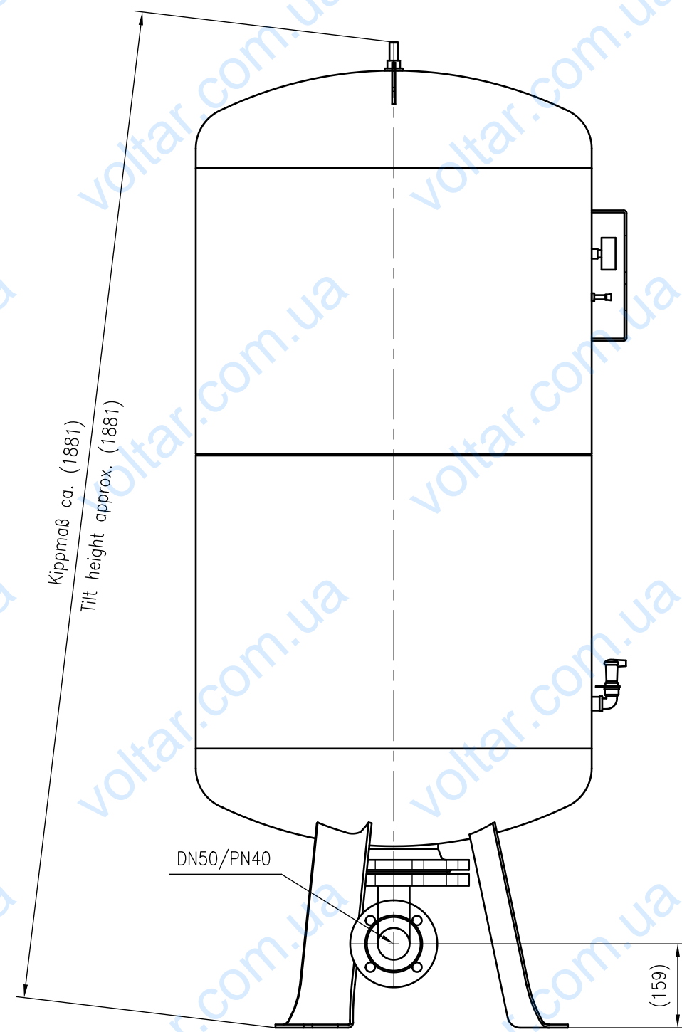
Side view
