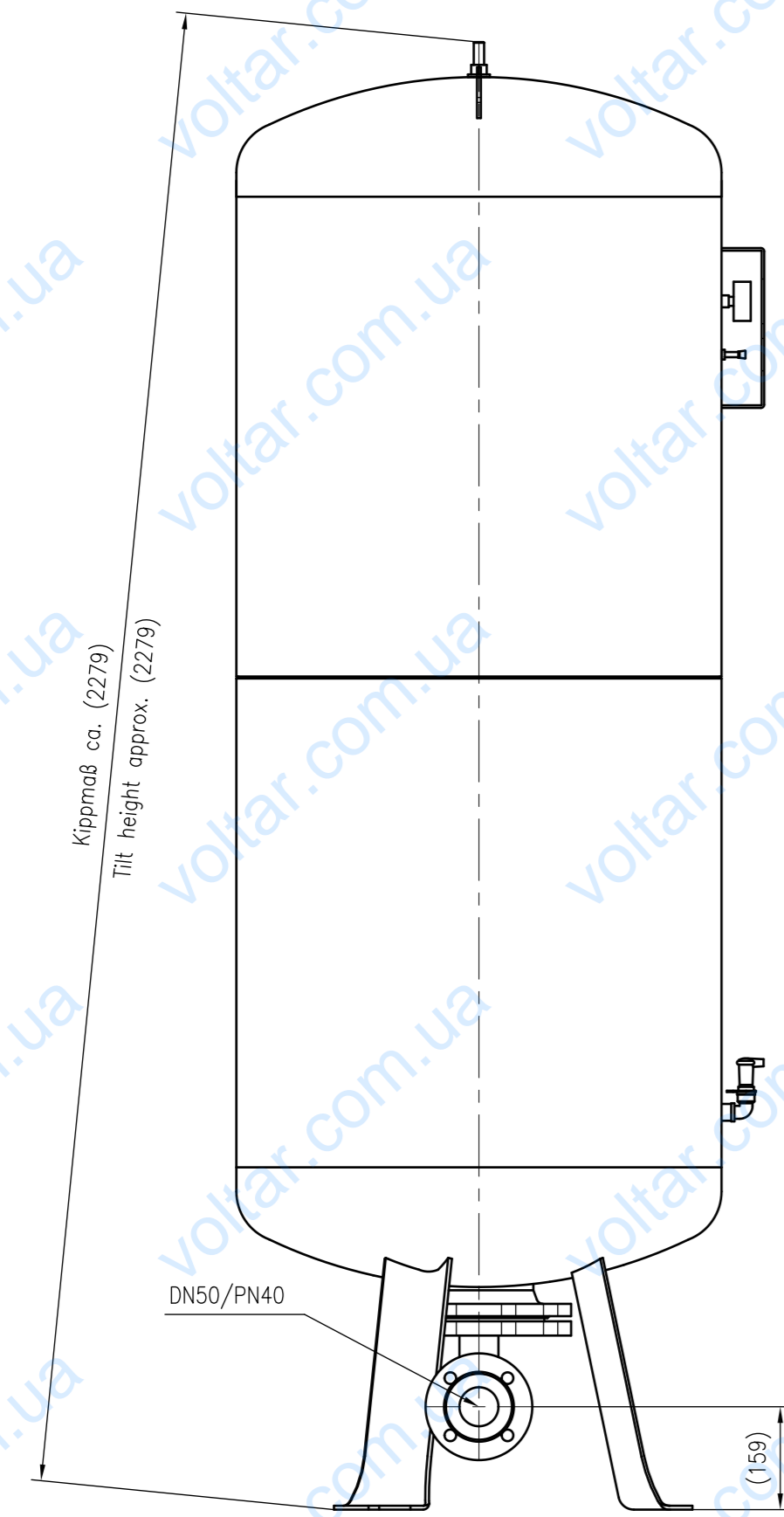
Side view
